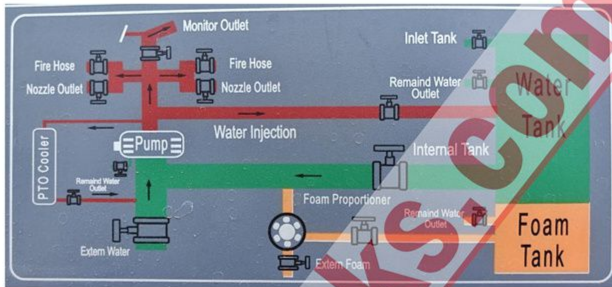
(Working Principle for fire truck)
